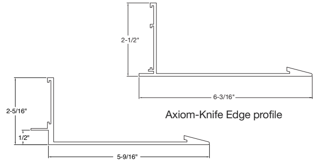
Axiom-Knife Edge for Vector profile
